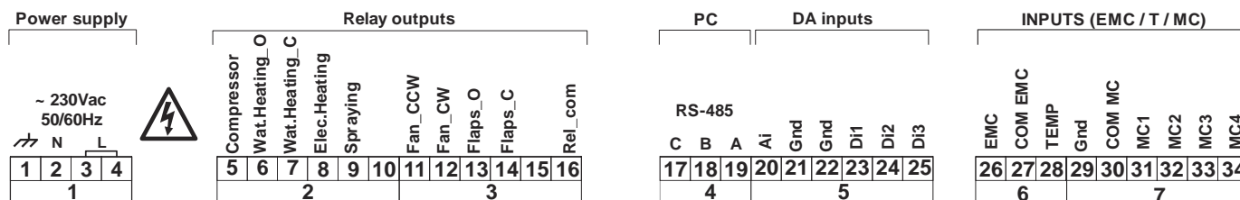
Picture 2.2. MC-904 clamps layout
